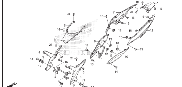
F-23-10 BODY COVER
