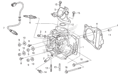
E-5 CYLINDER
