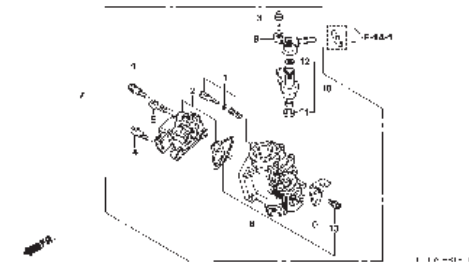
E-18 THROTTLE BODY
