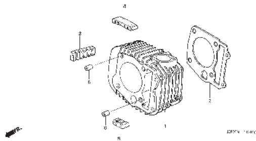
E-4 CYLINDER
