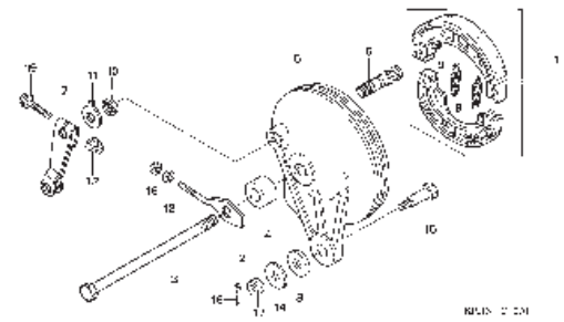
REAR BRAKE PANEL
