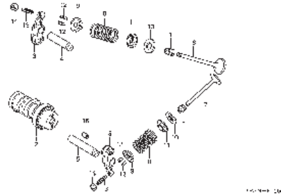
E-2 CAMSHAFT/VALVE
