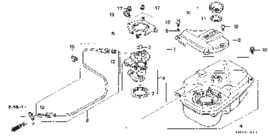
FUEL TANK
