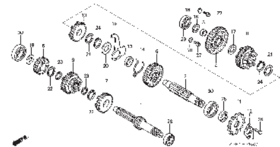
E-15 TRANSMISSION
