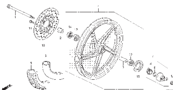
F-14-40 FRONT WHEEL(CAST)
