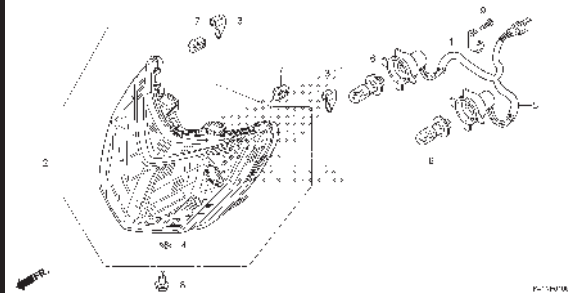
F-1 HEADLIGHT
