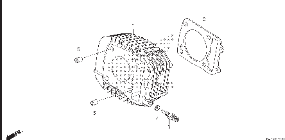
E-5 CYLINDER
