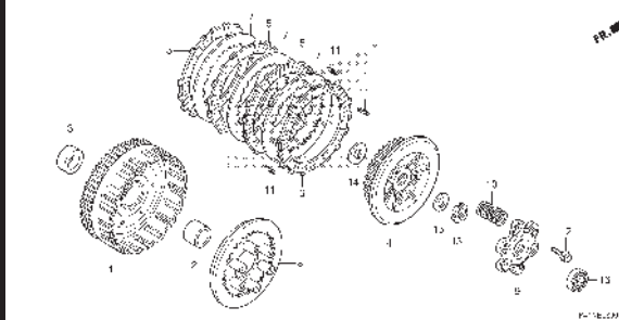
E-8 CLUTCH
