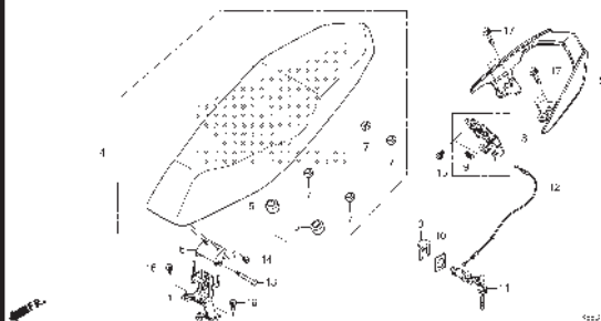
F-23 SEAT
