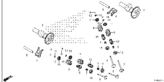
E-3 CAMSHAFT/VALVE
