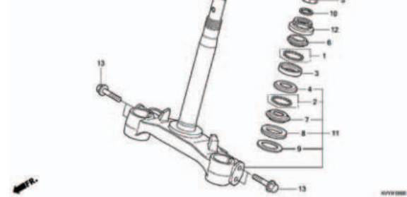
F-6 STEERING STEM
