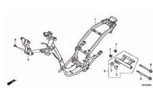
F-26 FRAME BODY
