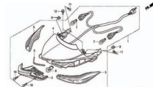
F-23 COMBINATION LIGHT
