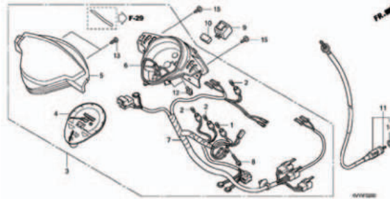
F-2 SPEEDOMETER
