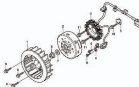
E-8 GENERATOR
