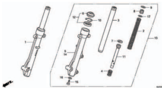
F-11 FRONT FORK
