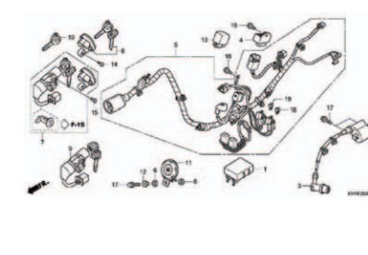
F-25 WIRE HARNESS
