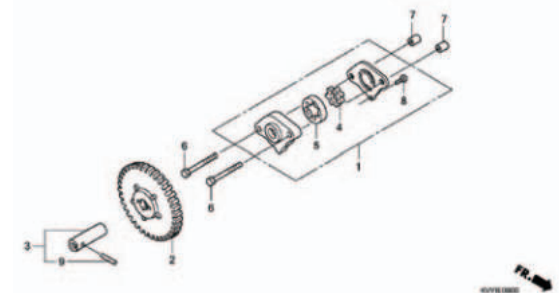
E-9 OIL PUMP
