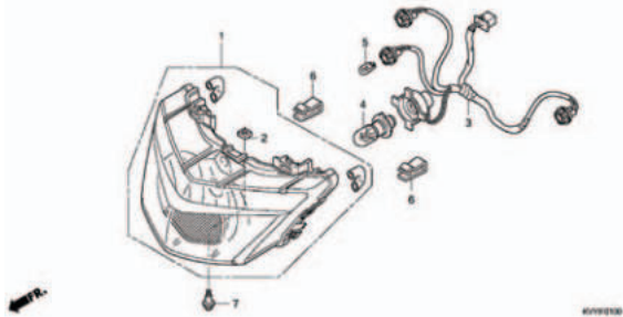
F-1 HEADLIGHT
