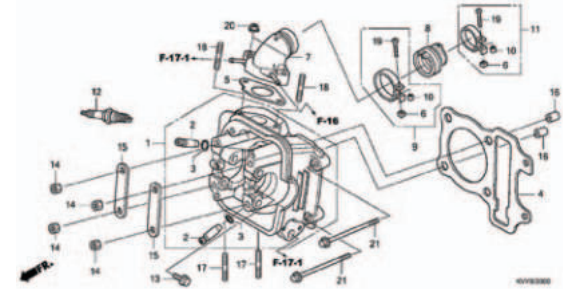
E-3 CYLINDER HEAD
