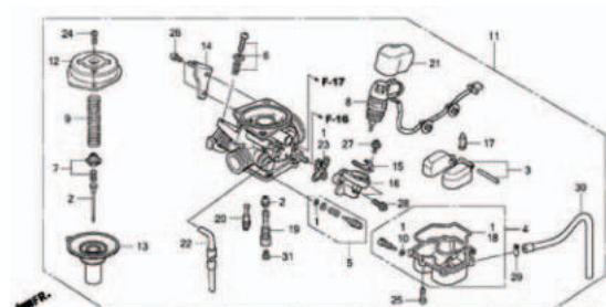
E-17 CARBURETOR
