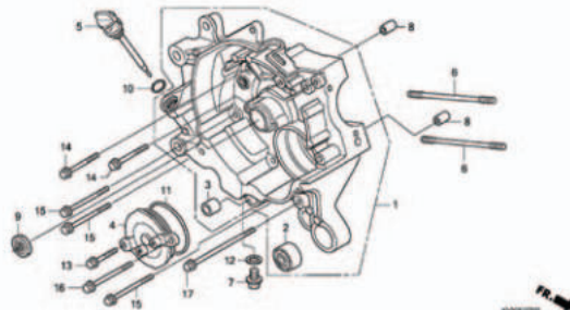
E-7 RIGHT CRANKCASE
