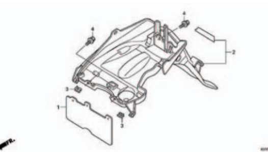
F-21 REAR FENDER
