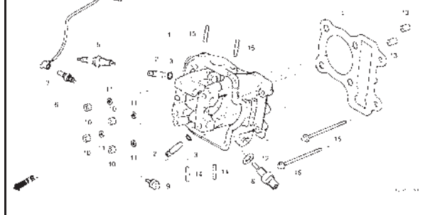
E-6 CYLINDER
