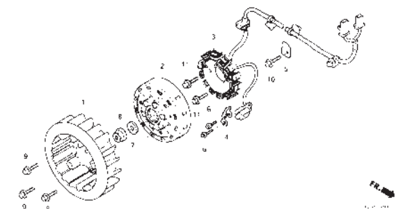
E-8 GENERATOR
