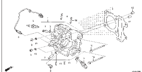
E-6 CYLINDER
