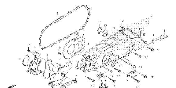
E-13 LEFT CRANKCASE COVER
