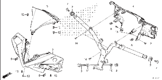
F-12 FRONT COVER/INNER COVER (ACH110CBF)
