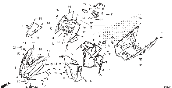
F-12-1 FRONT COVER/INNER COVER (ACH110CBT)
