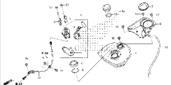
F-26 FUEL TANK/FUEL PUMP
