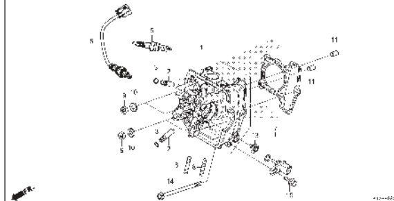
E-6 CYLINDER
