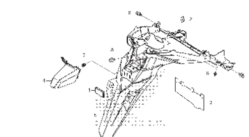
F-39 REAR FENDER
