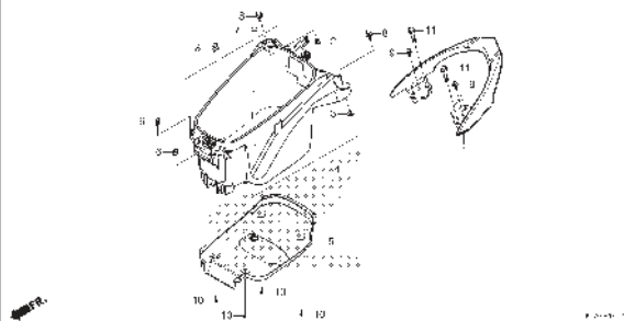
F-16 LUGGAGE BOX/GRAB RAIL
