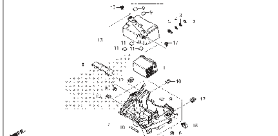
F-40 BATTERY
