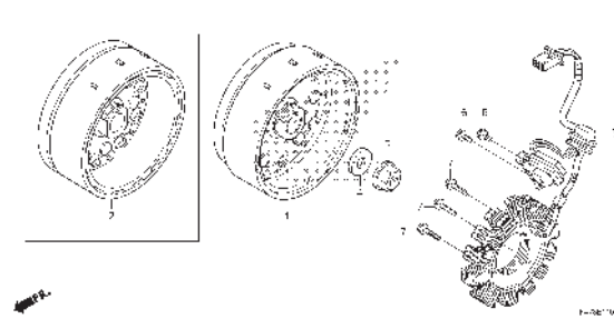
E-11 GENERATOR/FLYWHEEL
