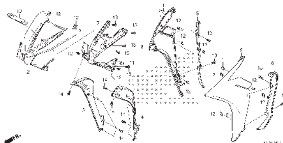
F-44 FRONT COVER/LEG SHIELD
