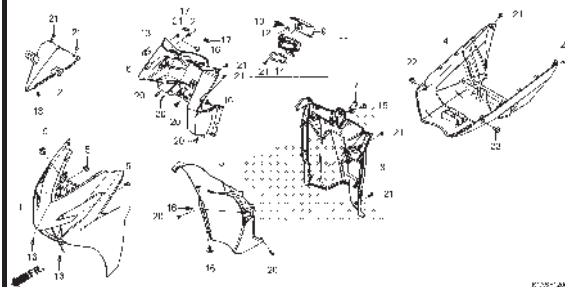
F-12 FRONT COVER/INNER COVER
