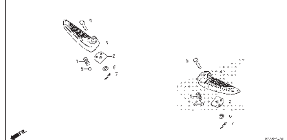
F-14-10 PILLION STEP (TIPE STREET)
