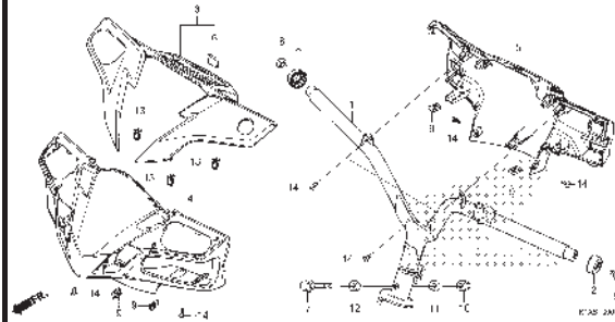
F-9-1 HANDLE PIPE/HANDLE COVER (TIPE CBS/CBS ISS)
