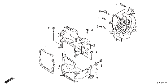
E-1 SHROUD/FAN COVER (CARBURETOR)
