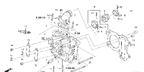
E-3 CYLINDER HEAD (CARBURETOR)
