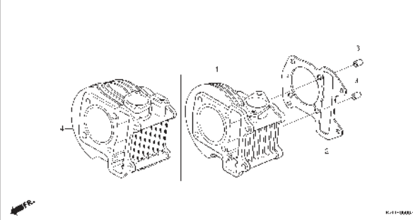
E-6 CYLINDER
