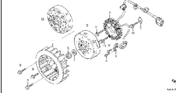
E-8 GENERATOR
