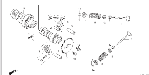
E-4 CAMSHAFT/VALVE
