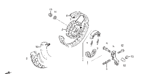
F-22-10 REAR WHEEL (SPOKE)
