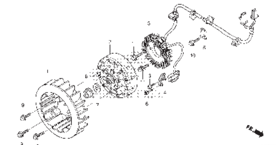
E-8 GENERATOR
