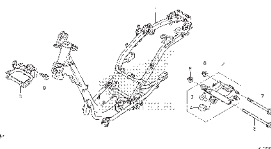
F-42 FRAME BODY
