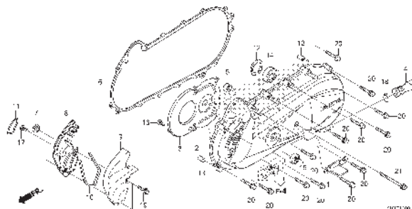
E-13 LEFT CRANKCASE COVER (ACF110CSFD/E)
