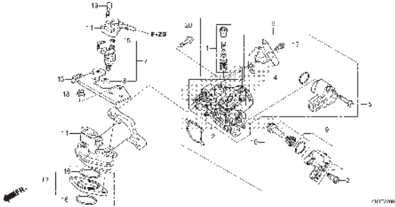
E-22 THROTTLE BODY(ACF110CSFD/E)
