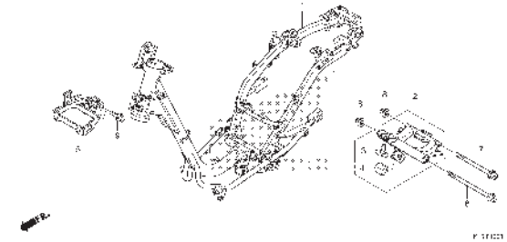
F-48 MARK(1)
