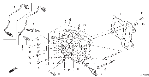
E-6 CYLINDER
