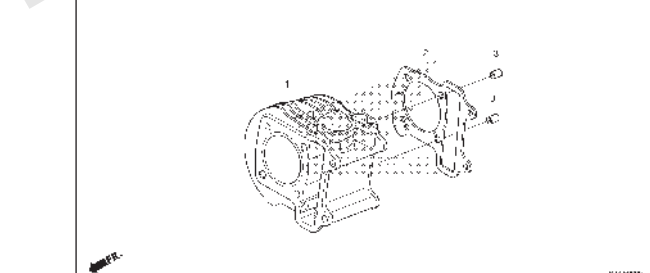
E-6 CYLINDER
