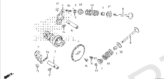
E-4 CAMSHAFT/VALVE
