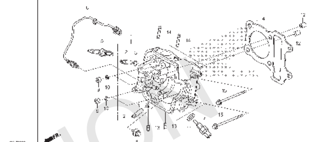
E-6 CYLINDER
