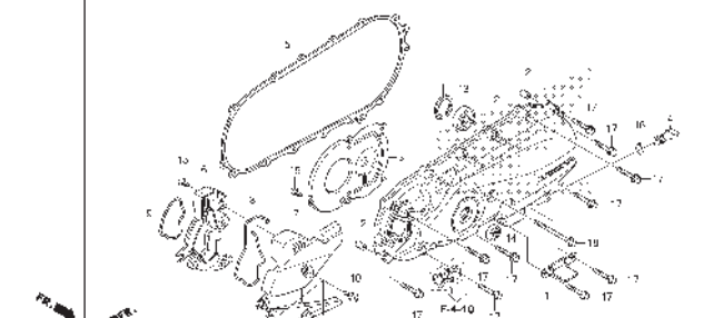
E-13 LEFT CRANKCASE COVER
