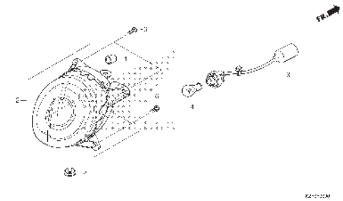
F-41 WIRE HARNESS(ACF110CBT-IN,3IN)
