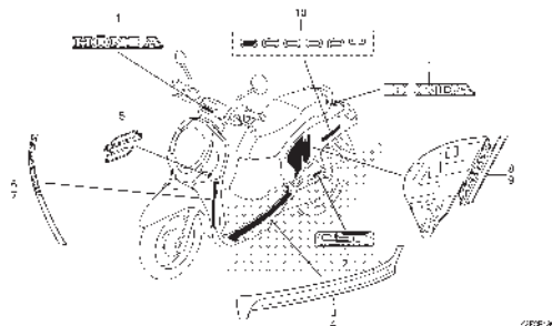
F-48 MARK/STRIPE(1)
