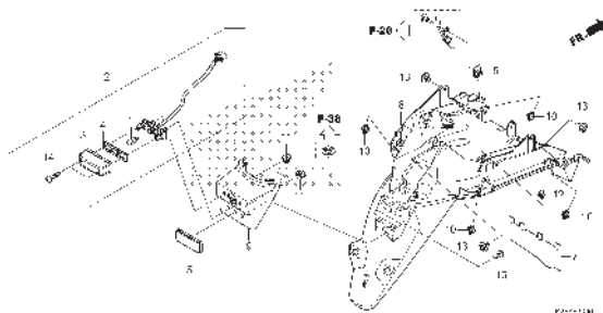
F-39 REAR FENDER
