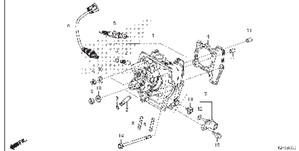
E-6 CYLINDER
