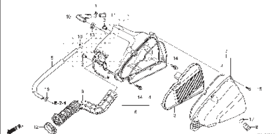
F-28-1 AIR CLEANER (ACI110CBG/H/J,CBTG/H/J)
