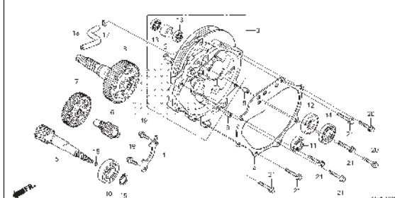
E-19-11 RIGHT CRANKCASE (ACI110CBG/H/J,CBTG/H/J)
