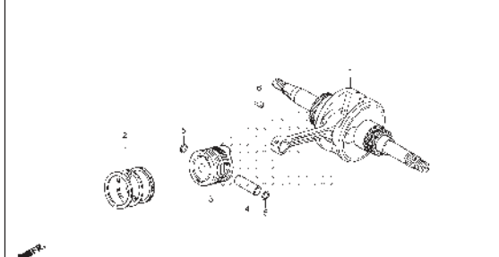
E-20 CRANKSHAFT/PISTON
