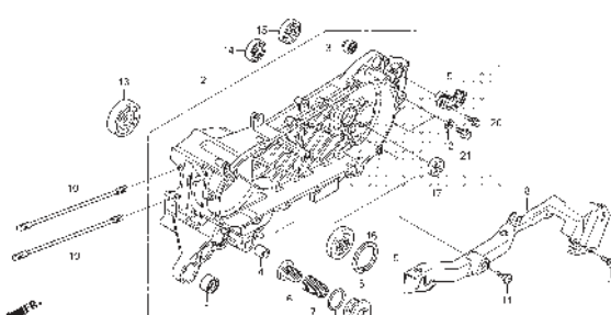
E-19-21 LEFT CRANKCASE (ACI110CBG/H/J,CBTG/H/J)
