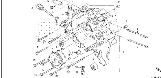
E-19-11 RIGHT CRANKCASE (ACI110CBG/H/J,CBTG/H/J)
