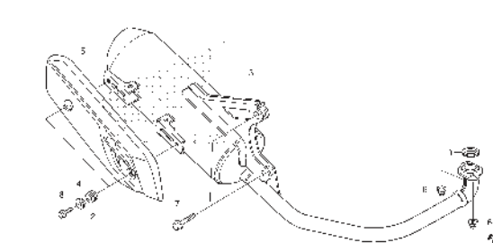
F-30 EXHAUST MUFFLER(ACI110CBE)
