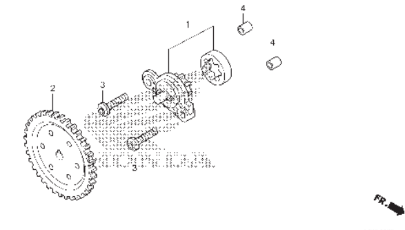
E-11 OIL PUMP
