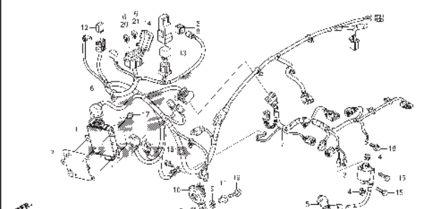
F-41 WIRE HARNESS
