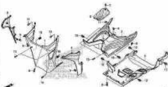
F-14-1 FLOOR STEP (ACB125CBFK/CBTK)
