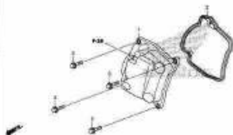
E-2 CYLINDER HEAD COVER (ACB125CBFF,G,J/CBTF,G,J)
