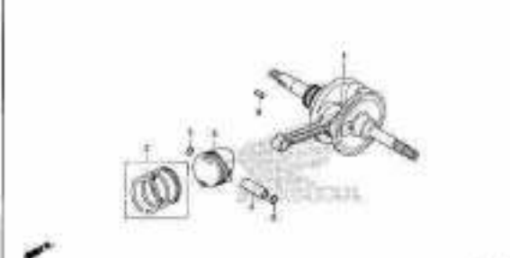
E-20 CRANKSHAFT/PISTON
