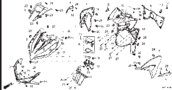
F-12-1 FRONT COVER(ACB125CBFP/CBTP)
