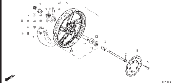
F-20-41 FRONT WHEEL(ACB125CBFP/CBTP)
