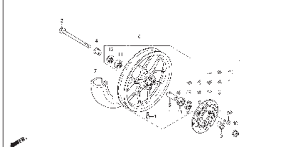
F-20-40 FRONT WHEEL (ACB125CBFL,M,N/CBTL,M,N)
