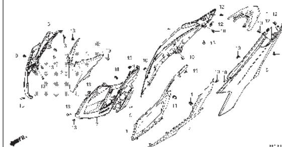
F-15-1 BODY COVER(ACB125CBFP/CBTP)
