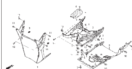
F-14-1 FLOOR STEP(ACB125CBFP/CBTP)
