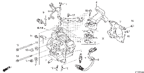
E-6 CYLINDER
