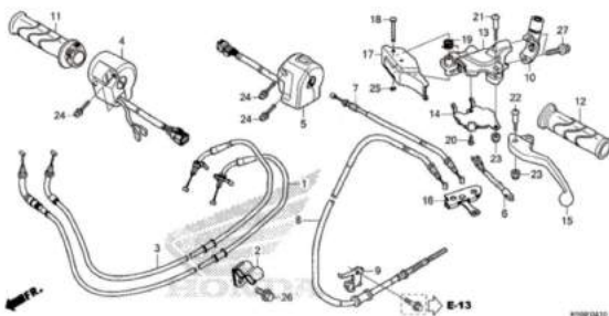
F-4-10 HANDLE LEVER/SWITCH/CABLE
