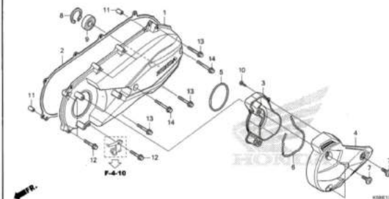
E-13 LEFT SIDE COVER
