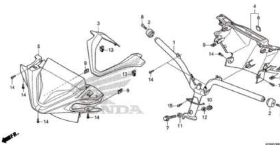
F-9 HANDLE PIPE/HANDLE COVER
