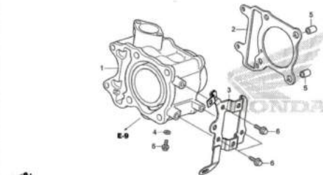
E-6 CYLINDER
