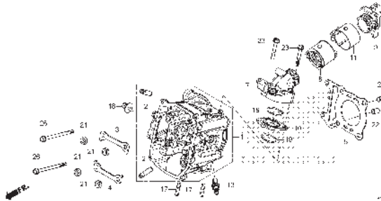
E-6 CYLINDER
