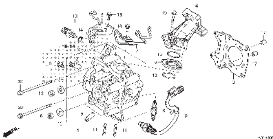
E-6 CYLINDER
