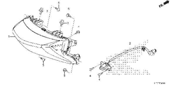
F-38-10 REAR COMBINATION LIGHT/ LICENSE LIGHT
