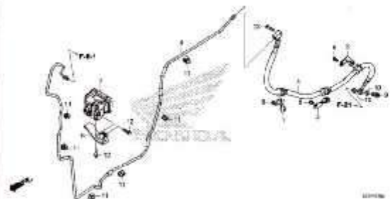
F-7-1 REAR BRAKE PIPE(WW150A)
