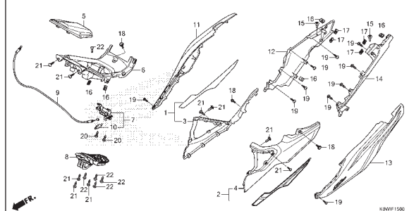
F-15 BODY COVER
