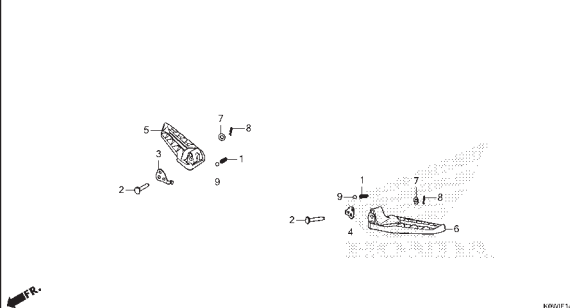
F-14-10 PILLION STEP
