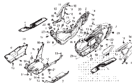
F-14 FLOOR STEP
