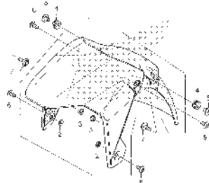
F-11 FRONT FENDER
