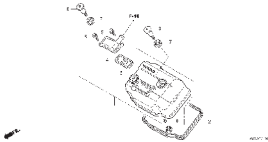
E-1 CYLINDER HEAD COVER
