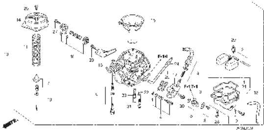
E-19 CARBURETOR
