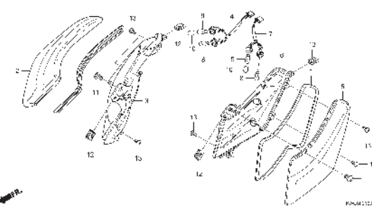
F-26 FRONT WINKER
