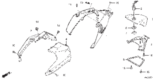
F-34 BODY COVER
