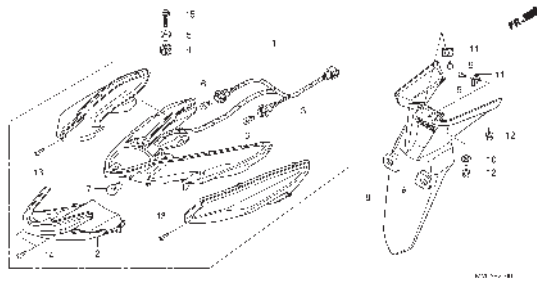
F-27 REAR COMBINATION LIGHT
