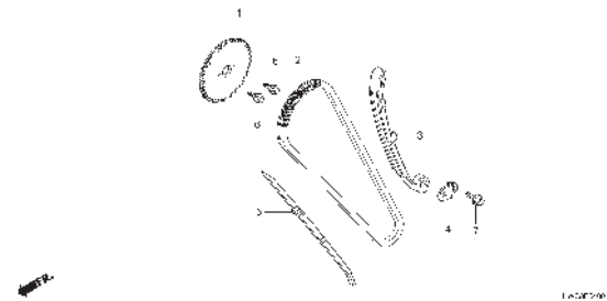
E-4 CAM CHAIN
