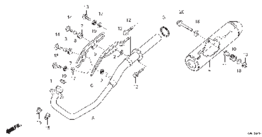
F-19 EXHAUST MUFFLER
