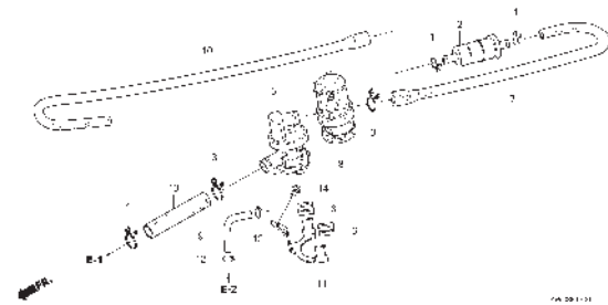
F-18 AIR INJECTION CONTROL VALVE
