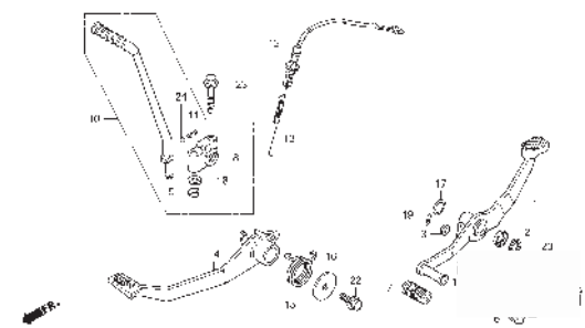
F-20 PEDAL/KICK STARTER ARM
