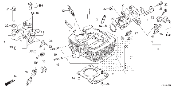
E-5 CYLINDER
