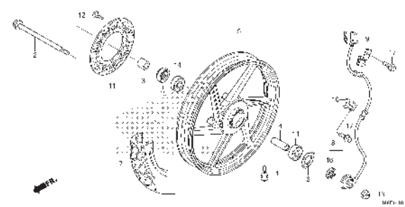
F-19-10 REAR WHEEL (TIPE CW)
