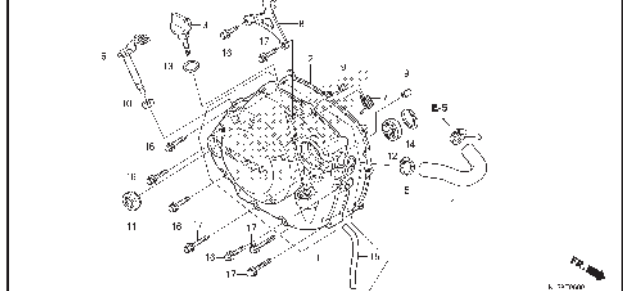
E-10 LEFT CRANKCASE COVER
