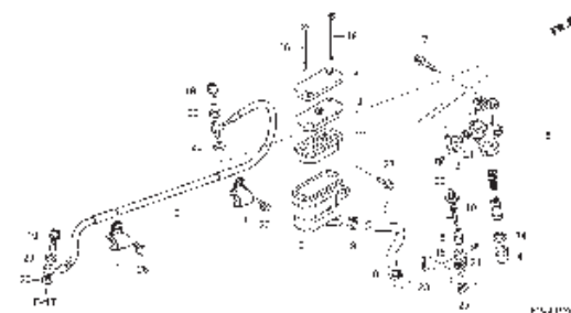
F-15 REAR BRAKE MASTER CYLINDER
