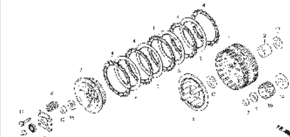
E-8 CLUTCH
