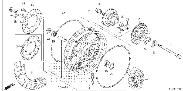
F-19-40 REAR WHEEL (CB150RG/H/J/K/L)
