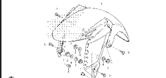
F-10-1 FRONT FENDER(CB150RM)
