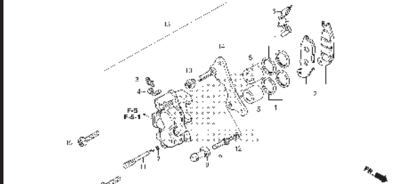
F-12-10 FRONT BRAKE CALIPER
