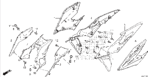
F-22 SHROUD(CB150RG/H/J)
