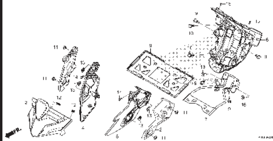
F-43-1 FRONT COWL(CB150RM)
