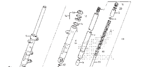
F-11 FRONT FORK(CB150RG/H/J/K/L)
