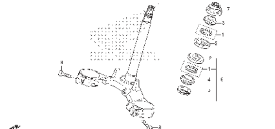
F-9-1 STEERING STEM(CB150RM)
