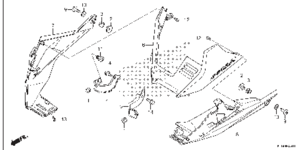
F-45-1 UNDER COWL(2)
