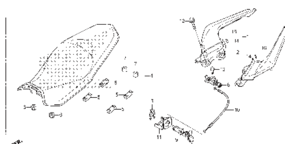
F-23 SEAT
