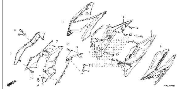
F-22-1 SHROUD(CB150RK/L)
