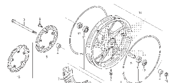
F-14-40 FRONT WHEEL (CB150RG/H/J/K/L)
