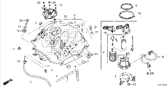
F-21 FUEL TANK (CB150RG/H/J/K/L)
