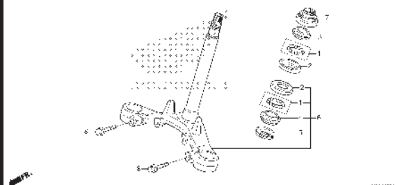
F-9 STEERING STEM (CB150RG/H/J/K/L)
