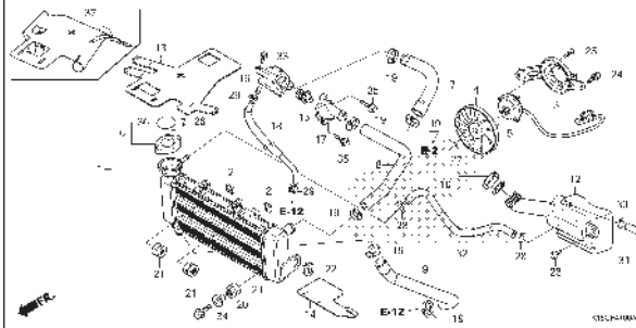
F-41 RADIATOR
