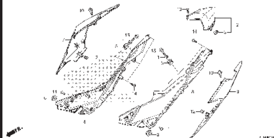
F-24-1 REAR COWL(CB150RK/L)
