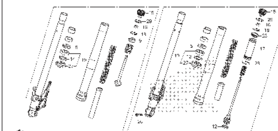
F-11-1 FRONT FORK(CB150RM)
