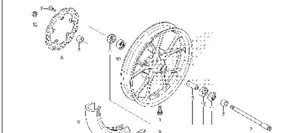
F-14-41 FRONT WHEEL (CB150RM)
