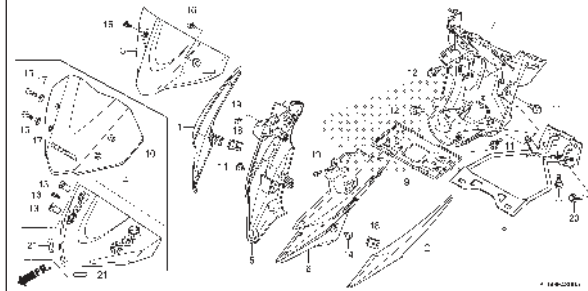
F-45-1 UNDER COWL(2)
