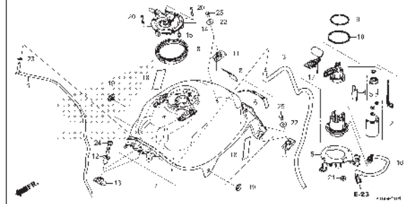
F-21-1 FUEL TANK(CB150RM)
