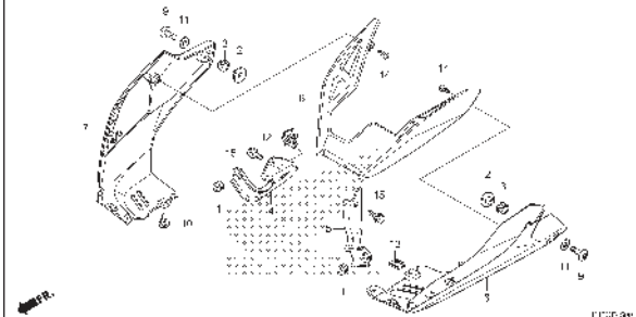
F-45 UNDER COWL(1)
