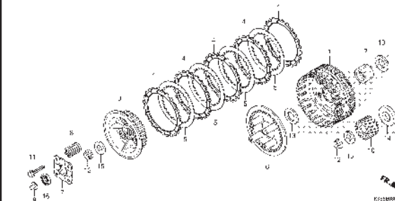
E-8 CLUTCH
