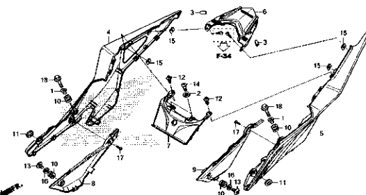
F-24 SIDE COVER/REAR COWL
