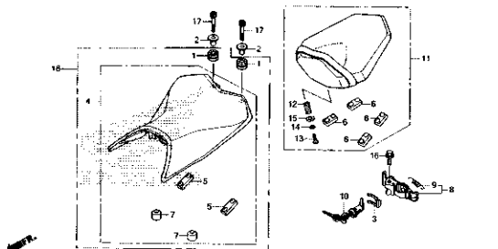
F-23 SEAT
