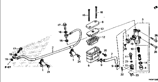
F-15 REAR BRAKE MASTER CYLINDER (CBR150R)
