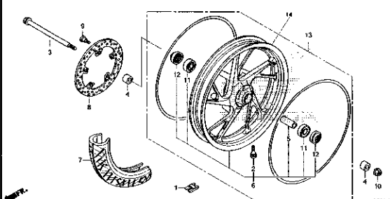
F-14-40 FRONT WHEEL(CBR150RG/J)
