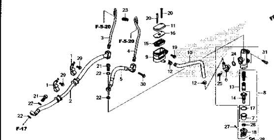
F-15-1 REAR BRAKE MASTER CYLINDER (CBR150RA)
