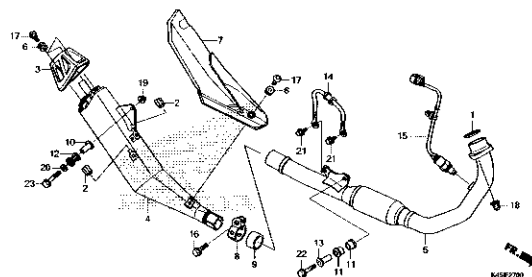
F-27 EXHAUST MUFFLER
