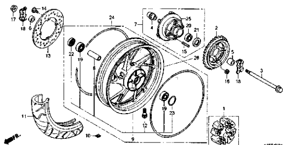
F-19-40 REAR WHEEL(CBR150RG/J)
