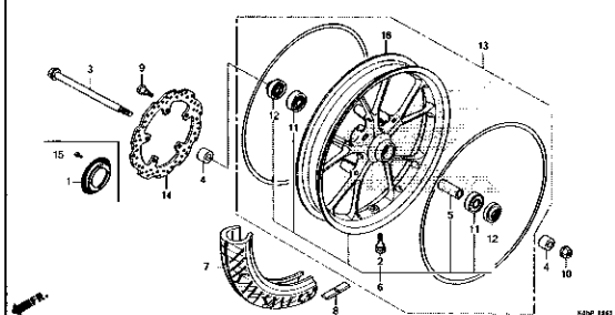
F-14-41 FRONT WHEEL(CBR150RK/RAK)
