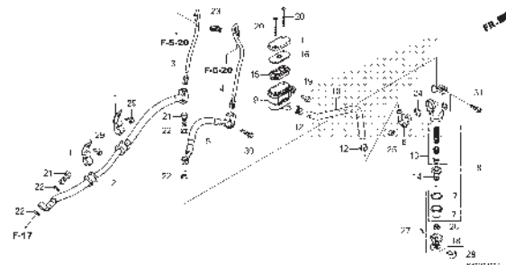
F-15-1 REAR BRAKE MASTER CYLINDER(CBR150RA)
