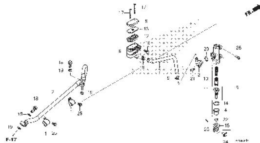
F-15 REAR BRAKE MASTER CYLINDER(CBR150R)
