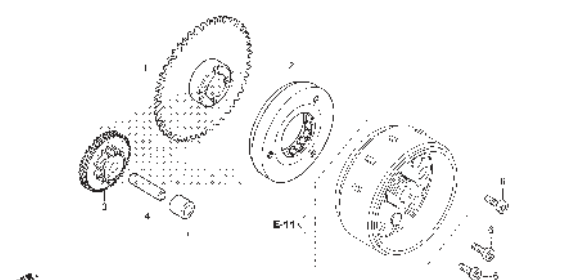
E-9 STARTING CLUTCH
