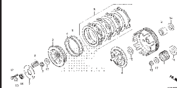
E-8 CLUTCH
