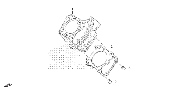
E-5 CYLINDER
