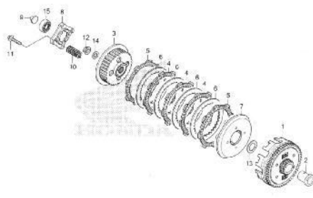
E-8 CLUTCH
